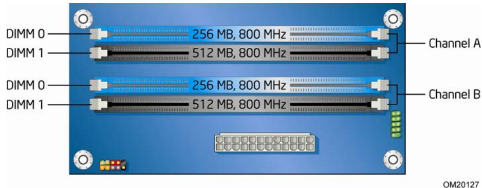
Figure 14. Dual Channel Memory Configuration with Four DIMMs
